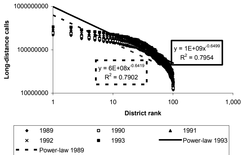
Fig. 11.7. Italian phone calls over time (1989–1993) and interpolating power laws
