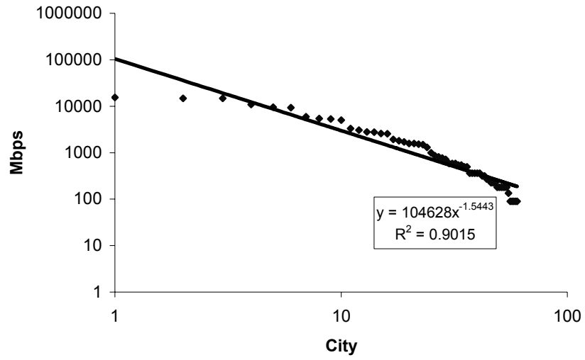
Fig. 11.2. Power-law distribution of the USA Internet 1998
