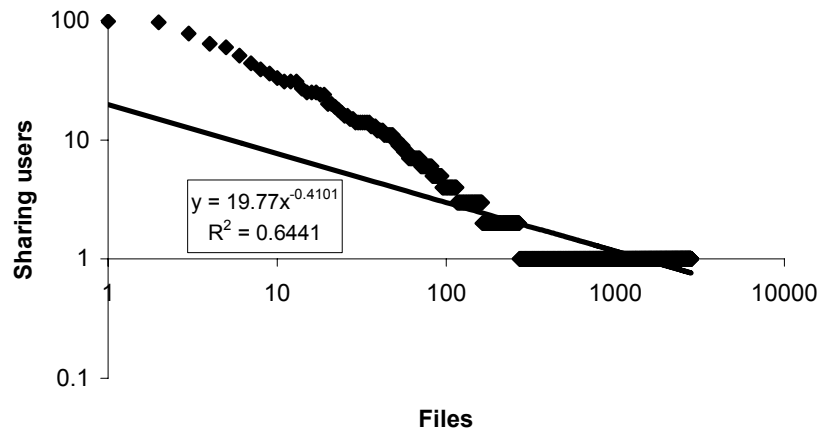
Fig. 11.9. Files' sharing comprising single-user shared files (2003)
