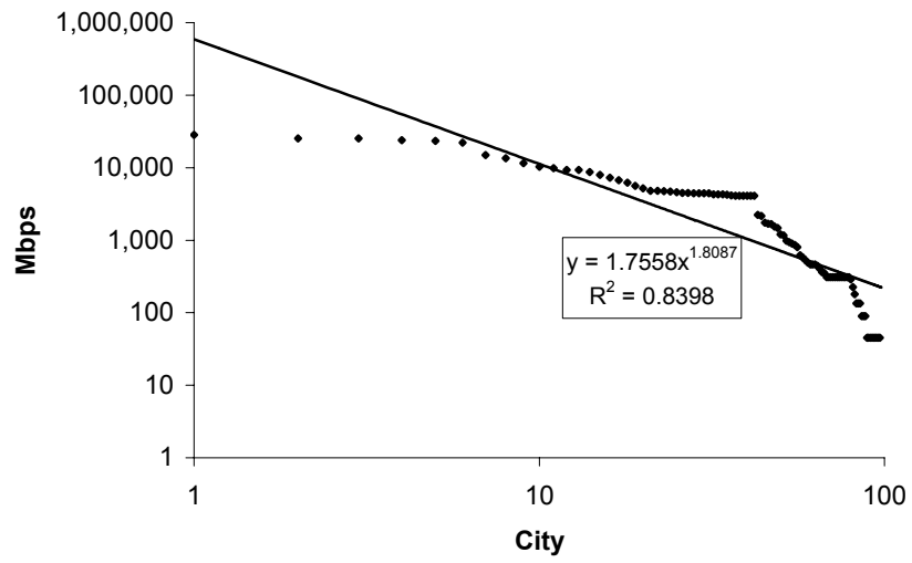
Fig. 11.3. Power-law distribution of the USA Internet 1999
