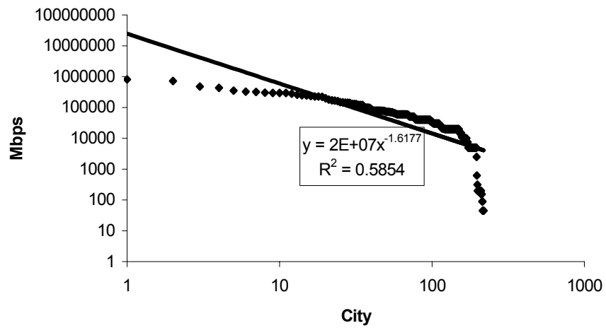
Fig. 11.5. Power-law distribution of the USA Internet 2003
