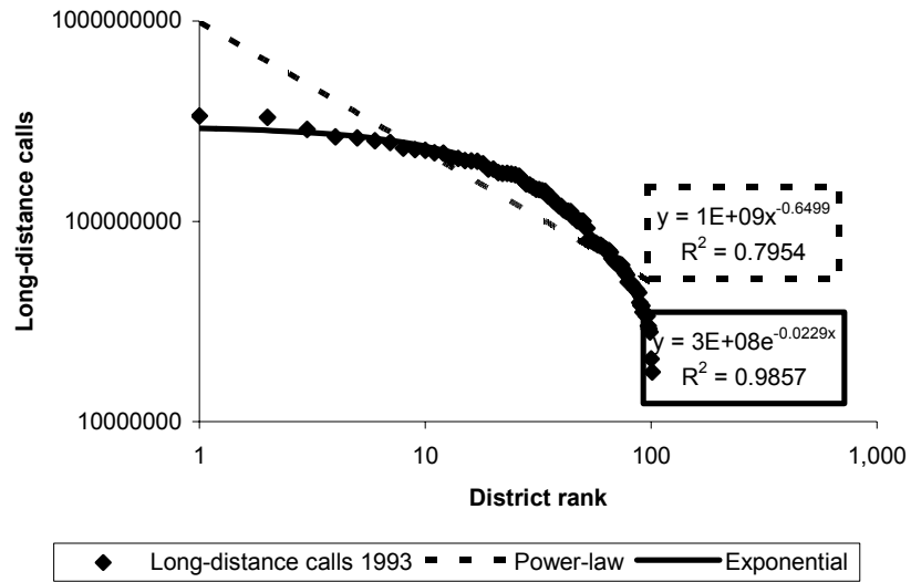
Fig. 11.6. Log-log plotting of Italian landline phone calls for 1993
