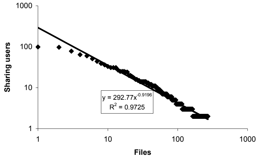
Fig. 11.8. Distribution of shared files over the network users (2003)
