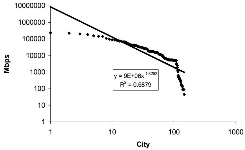
Fig. 11.4. Power-law distribution of the USA Internet 2000
