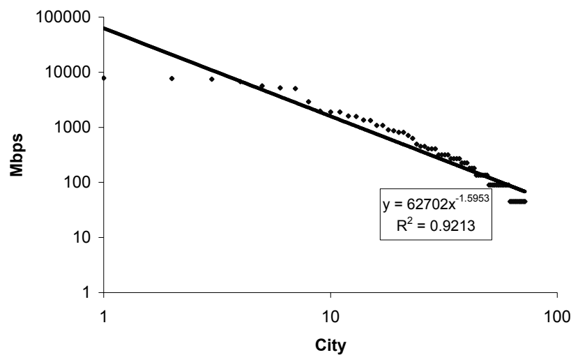
Fig. 11.1. Power-law distribution of the USA Internet 1997
